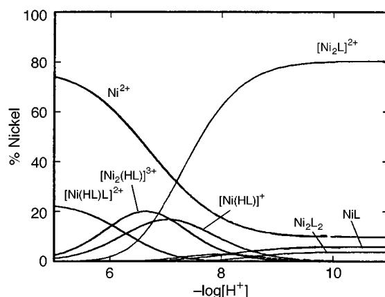
Fig. 2 Species distribution diagram as a function of -\log[H^+] for the sal- m -phen- Ni^{II} system at ligand:metal ratio 1:2 and c_M = 4 \times 10^{-3} mol dm -3 . Calculated from the \log K values given in Table 2
