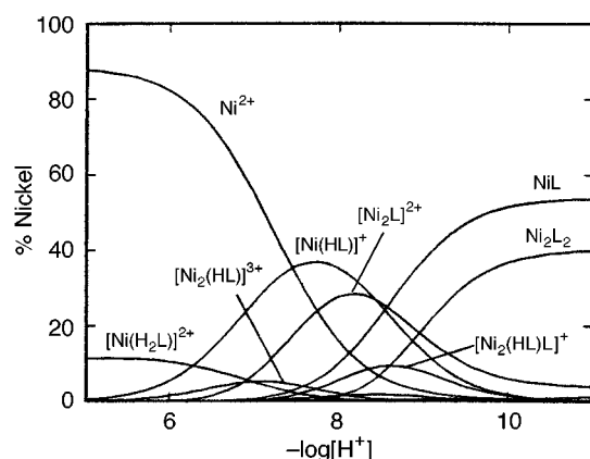
Fig. 1 Species distribution diagram as a function of -\log[H^+] for the sal- m -phen- Ni^{II} system at ligand:metal ratio 1:1 and c_M = 0.5 \times 10^{-3} mol dm -3 . Calculated from the values of \log K given in Table 2
