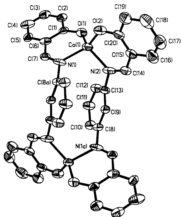
Fig. 3 An ORTEP view of the binuclear complex [Co_2(sal-m-phen)_2] showing the atom labelling. Thermal ellipsoids are drawn at the 50% probability level. Hydrogen atoms and chloroform molecules are omitted for clarity. Symmetry transformation related to a: -x + 1, -y, -z + 1
